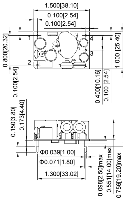
CFM12SXXX
