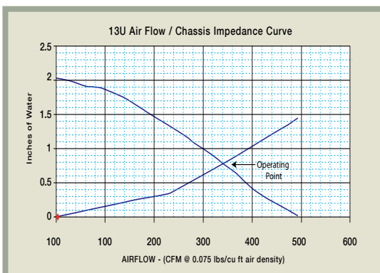
13U Airflow / Chasis Impedance Curve
